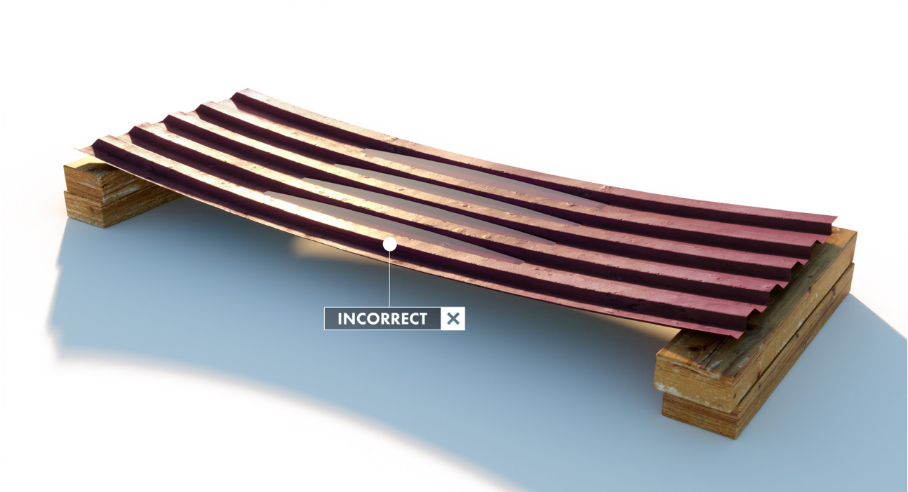
Insufficient support in the center of long panels allow "Bowing" or "Sagging" that traps water in the center of the panel length.
